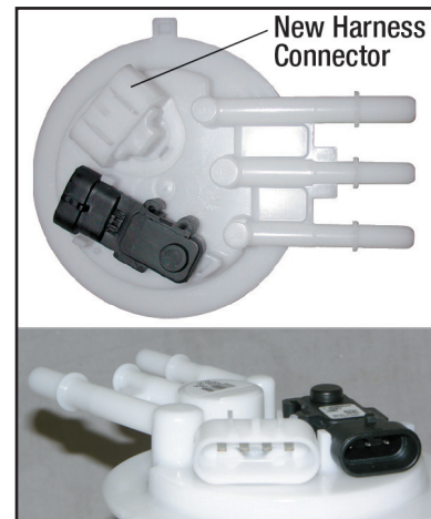
GM Fuel Pump Module with New Harness Connector
