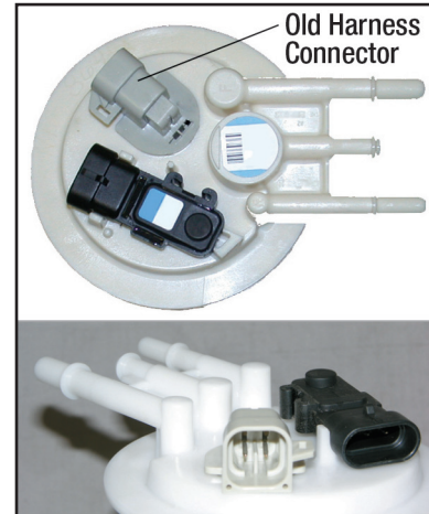
GM Fuel Pump Module with Old Harness Connector
